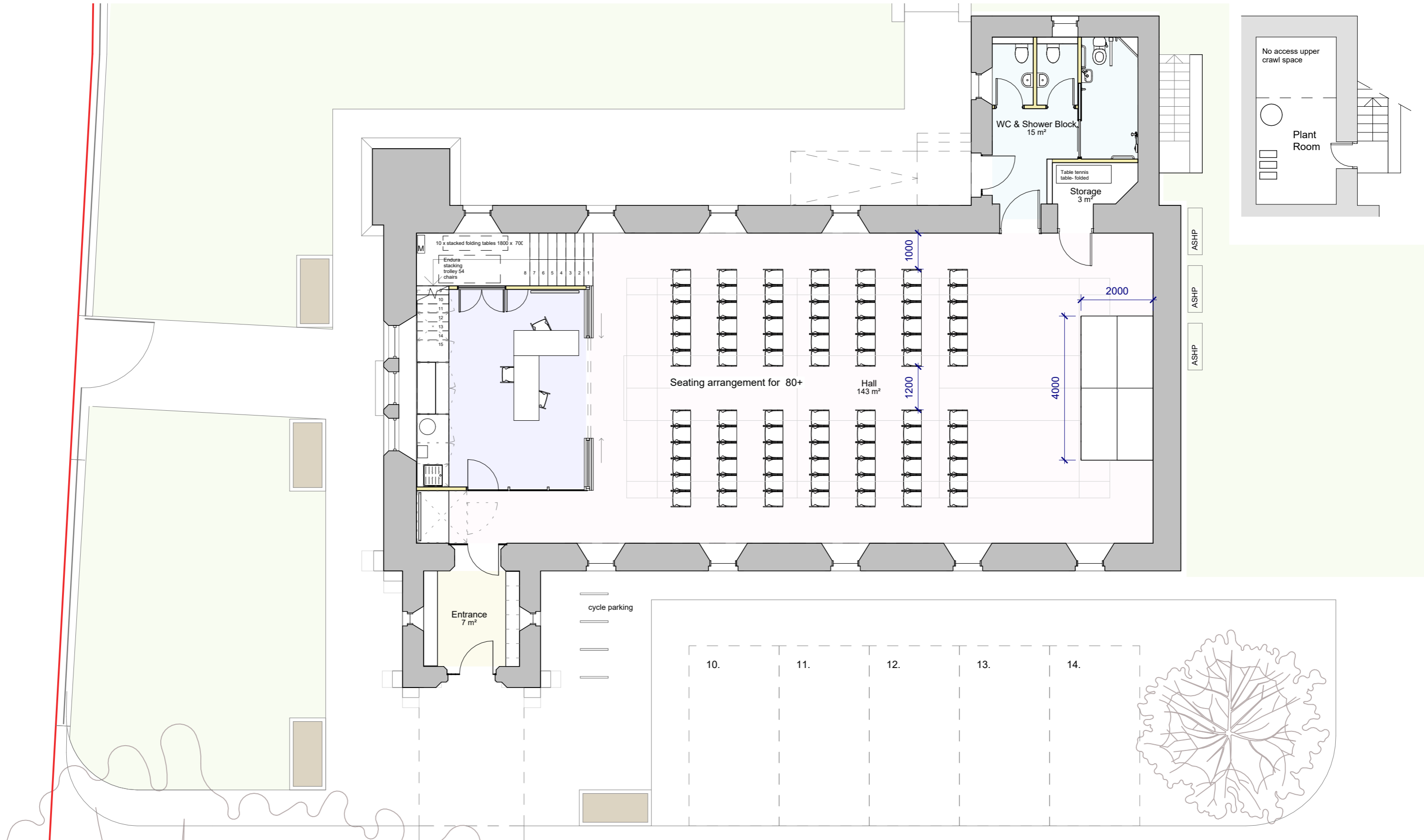
1 Proposed Ground Floor Level- Event Layout 1 : 100
