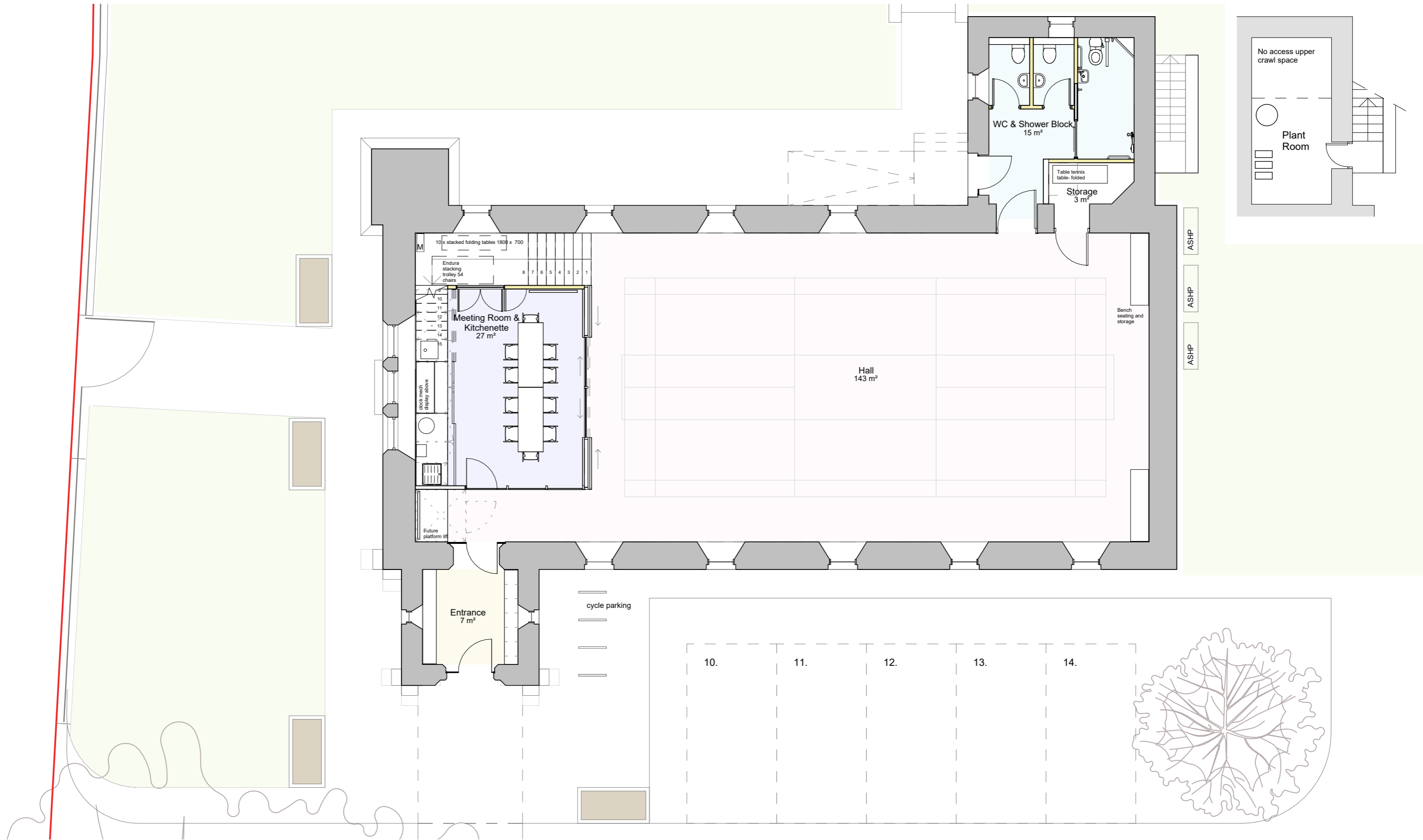
1 Proposed Ground Floor Level 1 : 100
